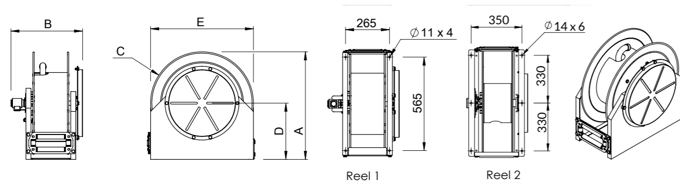
F-Series High Roller Hose Reel (F-Series High Roller Model)
