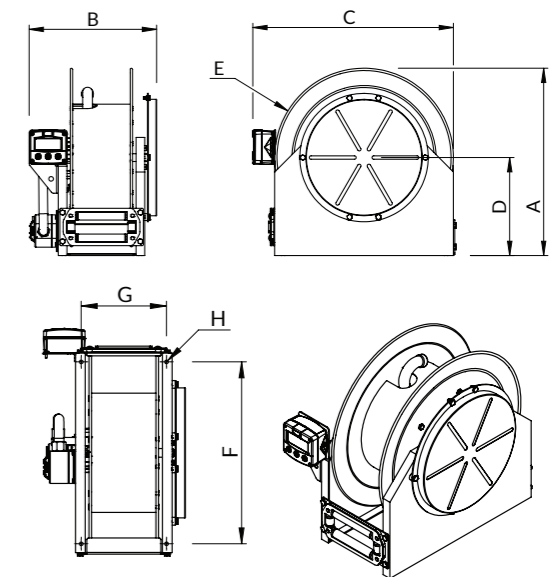
- 1" Metered Reel Illustrated - Dimensions are in mm
